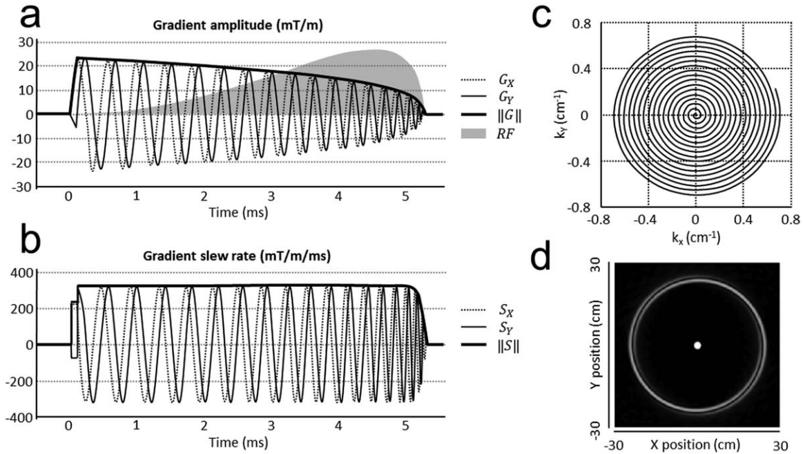
FIG. 1. a: Spiral-in gradient waveform (5.17 ms) generated using an exponential slew-rate recovery model (20) and RF shape (gray area, arbitrary units) exciting a 0.7-cm cylinder radius. b: Following hardware limitations, the gradient time-derivative shows that the gradient system is working in the slew-rate limited regime (330 mT/m/ms), and further constrained near the k-space center. c: Corresponding excitation k-space. The maximum extent in k-space k_{\max} and the interval between two consecutive spiral turns characterize the cylinder radius and position of the first aliasing lobes of the excitation profile. d: The simulated excitation profile (FA = 30°, FOV 30 × 30 cm 2 , arbitrary units).
