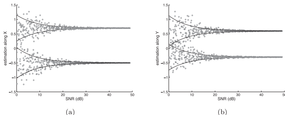
FIG. 6. 6(a) and 6(b) depict the lower bounds of any unbiased estimator (solid line) and some sample estimations (grey circles) obtained through our technique for x_i and y_i , respectively, with i \in \{1, 2\} . Moreover, we used the following four analytic sensors: \psi_{a_n} = \frac{1}{z - 1.1e^{i\frac{\pi}{2}n}} , with n \in \llbracket 0, 3 \rrbracket .
