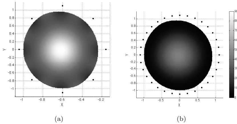
FIG. 8. 8(a) and 8(b) depict the sum of the minimal estimation errors, indicated by the gray-scale intensity, when shifting a dipole through a unit-disk using a squared grid with step 0.01. The displacement of the point source with intensity -1 with respect to the point source with intensity 1 is (-0.05, 0.1) and the dipole's intensity is 1 . The noise is Gaussian with expected value 0 and variance 0.06 . The analytic sensors are, respectively, \psi_{a_n} = (z - 1.1e^{in\frac{\pi}{4}})^{-1} with n \in \llbracket 0, 7 \rrbracket and \psi'_{a_n} = (z - 1.1e^{in\frac{\pi}{16}})^{-1} with n \in \llbracket 0, 31 \rrbracket .
