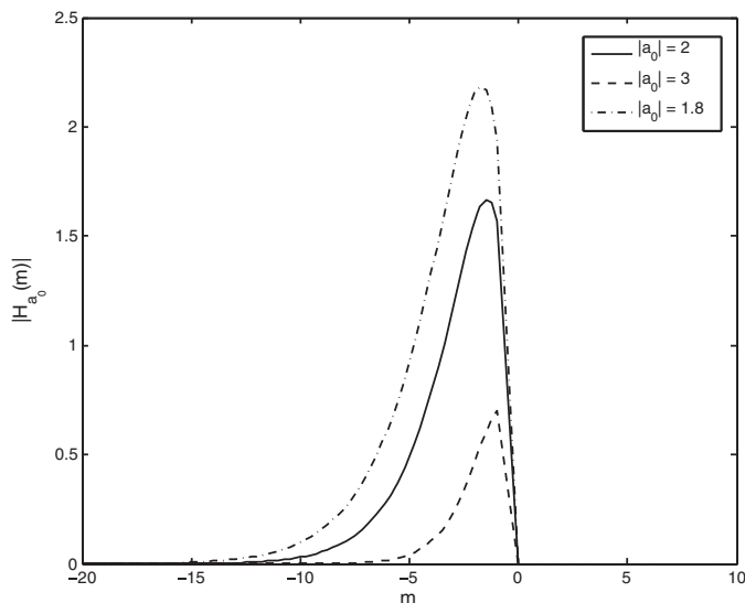
FIG. 3. Magnitude of the frequency response of H_{a_0}(m) that is the equivalent filter that links the boundary measures to the generalized measures. Different magnitudes of the pole a_0 are shown.
