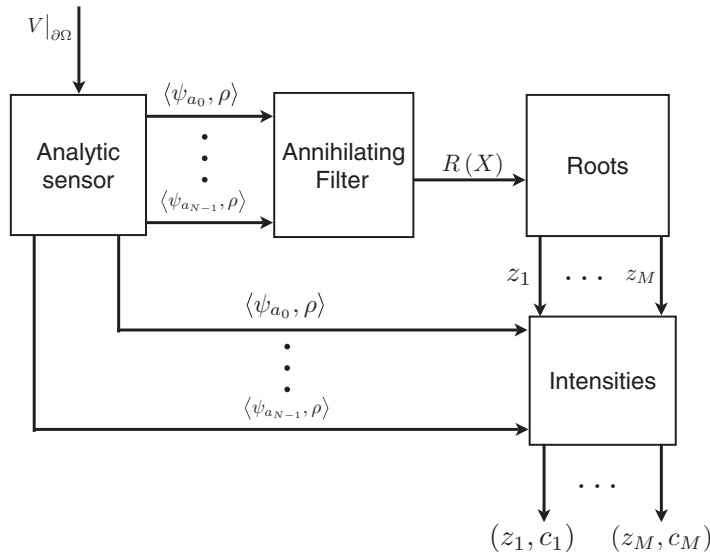
FIG. 4. A flow chart of the proposed algorithm to determine the positions of the pointwise sources and their corresponding intensities.
