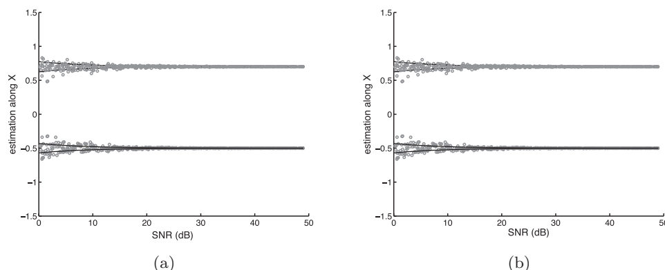
FIG. 7. 7(a) and 7(b) depict the lower bounds of any unbiased estimator (solid line) and some sample estimations (grey circles) obtained through our technique for x_i and y_i , respectively, with i \in \llbracket 1, 2 \rrbracket using the following 50 analytic sensors: \psi_{a_n} = \frac{1}{z - 1.1e^{i\frac{\pi}{25}n}} , with n \in \llbracket 0, 49 \rrbracket .
