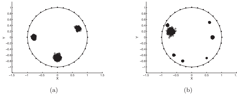
FIG. 9. 9(a) and 9(b) depict the localization of 3 and 7 point sources, respectively. The noise added to the generalized measures is Gaussian with zero mean such that the localization is performed at 15dB and 40dB, respectively. The analytic sensors are \psi'_{a_n} = (z - 1.01e^{in\frac{\pi}{16}})^{-1} with n \in \llbracket 0, 31 \rrbracket .
