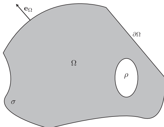
FIG. 1. A homogeneous 2D conductor \Omega with boundary \partial\Omega , source distribution \rho , constant conductivity \sigma , and outward surface normal \mathbf{e}_\Omega .
