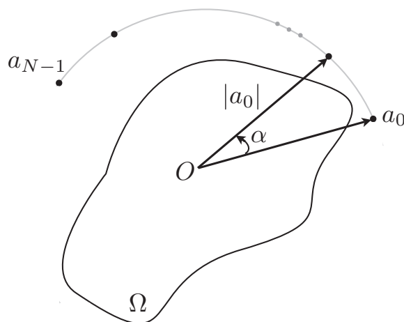
FIG. 2. The poles, a_0 \cdots a_{N-1} , and their placement outside of \Omega . For each pole there is a corresponding analytic sensor \psi_{a_n}(z) = \frac{1}{z - a_n} .
