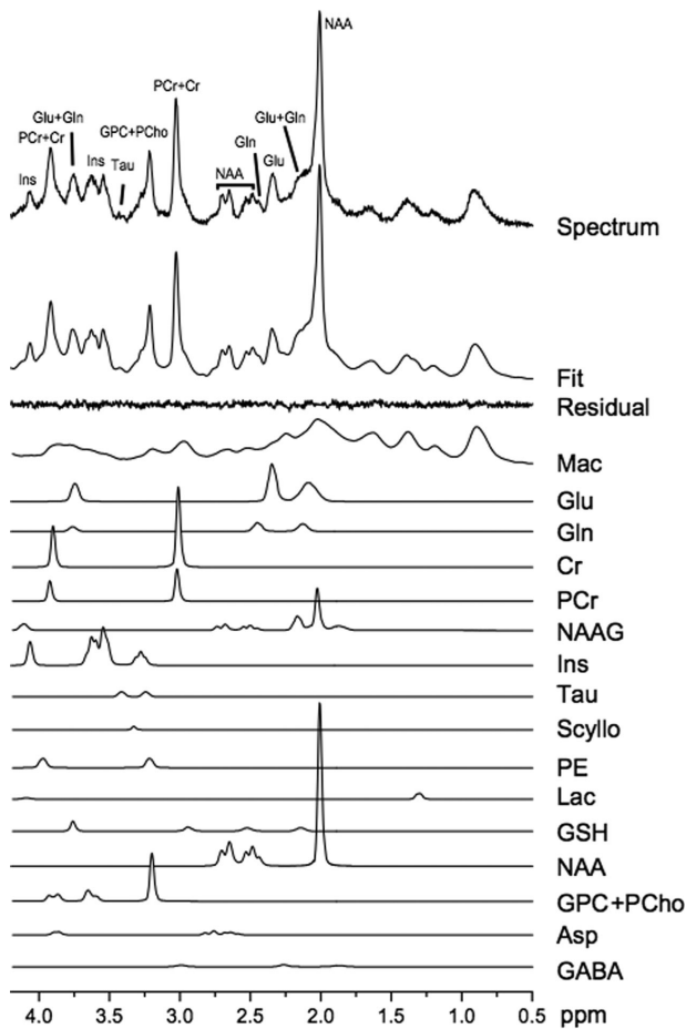
Fig 7. In vivo ^1\text{H} MR spectrum acquired using semiadiabatic SPECIAL localization sequence ( TE/TR = 12/7,500 milliseconds, 32 averages) from a volume of interest ( 20 \times 15 \times 20 \text{ mm}^3 ) in the occipital lobe of a healthy volunteer and its LC model fit, fit residual, and the individual metabolite fits. Lac = lactate; GABA = gamma-amino butyric acid; NAA = N-acetylaspartate; Glu = glutamate; Gln = glutamine; Asp = aspartate; Cr = creatine; PCr = phosphocreatine; GPC = glycerophosphocholine; Tau = taurine; Ins = myo-inositol; GSH = glutathione; PCho = phosphocholine; NAAG = N-Acetylaspartylglutamate; PE = phosphoethanolamine; Mac = macromolecule baseline. Numbers on the graph express the resonant frequencies in parts per million (ppm).
