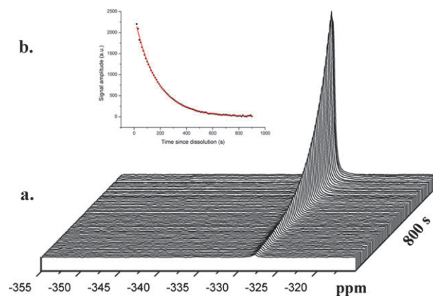
Fig. 2 (a) Series of spectra of hyperpolarized in vitro ^{15}\text{N} Cho measured in a phantom. The signal is visible up to \sim 800 – 900 s after dissolution. Individual spectra were processed with 10 Hz Lorentzian line broadening. The ^{15}\text{N} chemical shifts were referenced to nitromethane. (b) Decay curve of the same in vitro signal amplitudes (black dots) corrected for the RF flip angle effects. The fit of the plotted decay curve is also shown (line).
