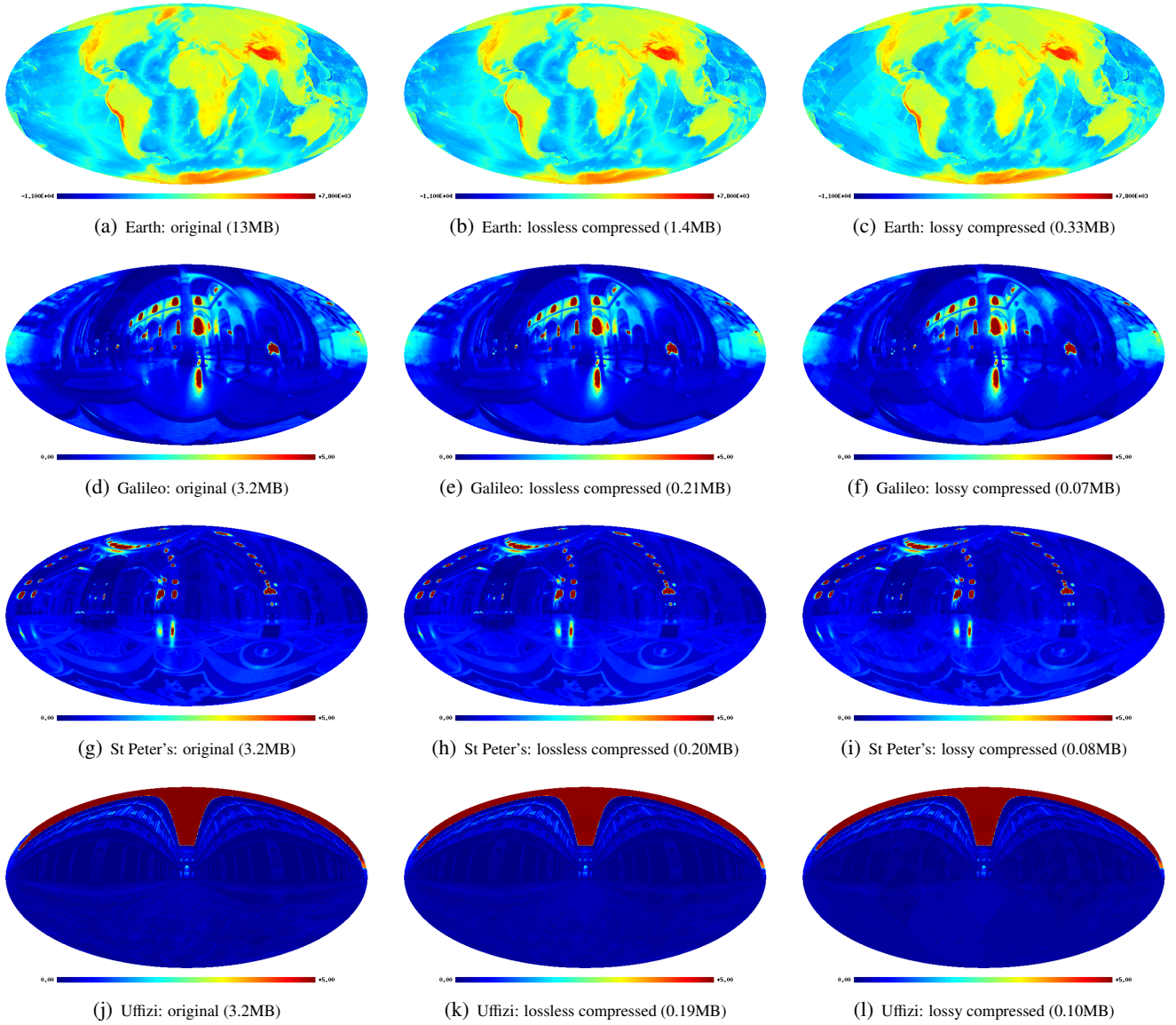
Figure 6. Compressed data for lossy compression applications. Each row of panels shows the original, lossless and lossy compressed data-spheres. File sizes for each data-sphere are also specified. The lossless compressed data shown in the second column of panels is performed with a precision parameter of p = 3 . The lossy compressed data shown in the third column of panels is performed by retaining 5% of detail coefficients only and including a RLE stage. The full dynamic range of these images may not be visible in printed versions of this figure, hence this figure is best viewed online.
