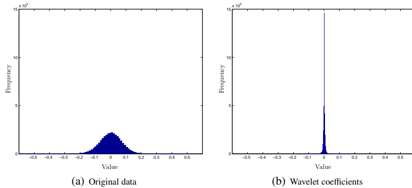
Figure 3. Histograms of original data and wavelet (approximation and detail) coefficient values. Although the particular data-sphere considered here is not important for the purpose of this demonstration, these histograms correspond to the CMB data described in Sec. 3.1. Notice how the Haar wavelet transform has compressed the energy content of the signal, thereby reducing its entropy and allowing for greater compression performance.
