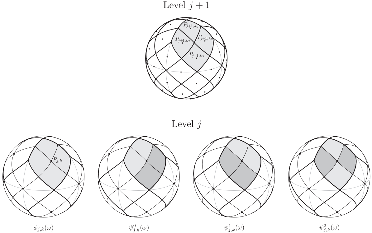
Figure 1. Haar scaling function \phi_{j,k}(\omega) and wavelets \psi_{j,k}^m(\omega) . Dark shaded regions correspond to negative constant values, light shaded regions correspond to positive constant values and unshaded regions correspond to zero. The scaling function and wavelets at level j and position k are non-zero on pixel P_{j,k} only. Pixel P_{j,k} at level j is subdivided into four pixels at level j + 1 , which we label P_{j+1,k_0} , P_{j+1,k_1} , P_{j+1,k_2} and P_{j+1,k_3} as defined above.
