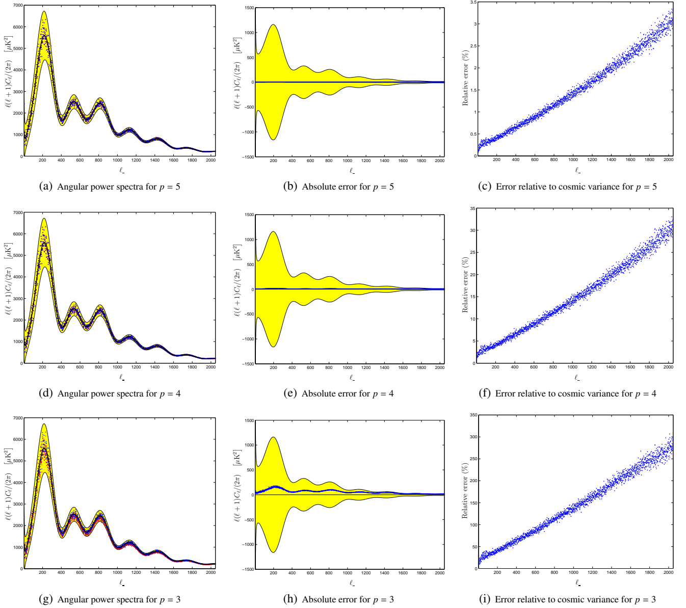
Figure 5. Reconstructed angular power spectrum of compressed CMB data. Each row of panels shows the reconstructed power spectrum and errors for a particular compression precision parameter p . In the first column of panels, the power spectrum reconstructed from the original CMB data are given by the red dots, the power spectrum reconstructed from the compressed CMB data are given by the blue dots and the underlying power spectrum of the simulated model is shown by the solid black line, with three standard deviation cosmic variance regions shaded in yellow. Note that in some instances the red and blue dots align closely and may not both be visible. In the second column of panels, the absolute error between the power spectra reconstructed from the original and compressed CMB data is given by the blue dots, with three standard deviation cosmic variance regions shaded in yellow. In the third column of panels, the absolute error between the power spectra reconstructed from the original and compressed CMB data is expressed as a percentage of cosmic variance. Note that the scale of the vertical axis changes by an order of magnitude between each row of the third column of panels.
