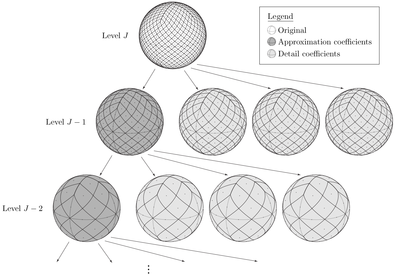
Figure 2. Haar multiresolution decomposition. Starting at the finest level J (the original data-sphere), the approximation and detail coefficients at level J-1 are computed. This procedure is repeated to decompose the approximation coefficients at level J-1 (i.e. the approximation function f_{J-1} ), into approximation and detail coefficients at the coarser level J-2 . Repeating this procedure continually, one recovers the multiresolution representation of f_J in terms of the coarsest level approximation f_{J_0} and all of the detail coefficients.
