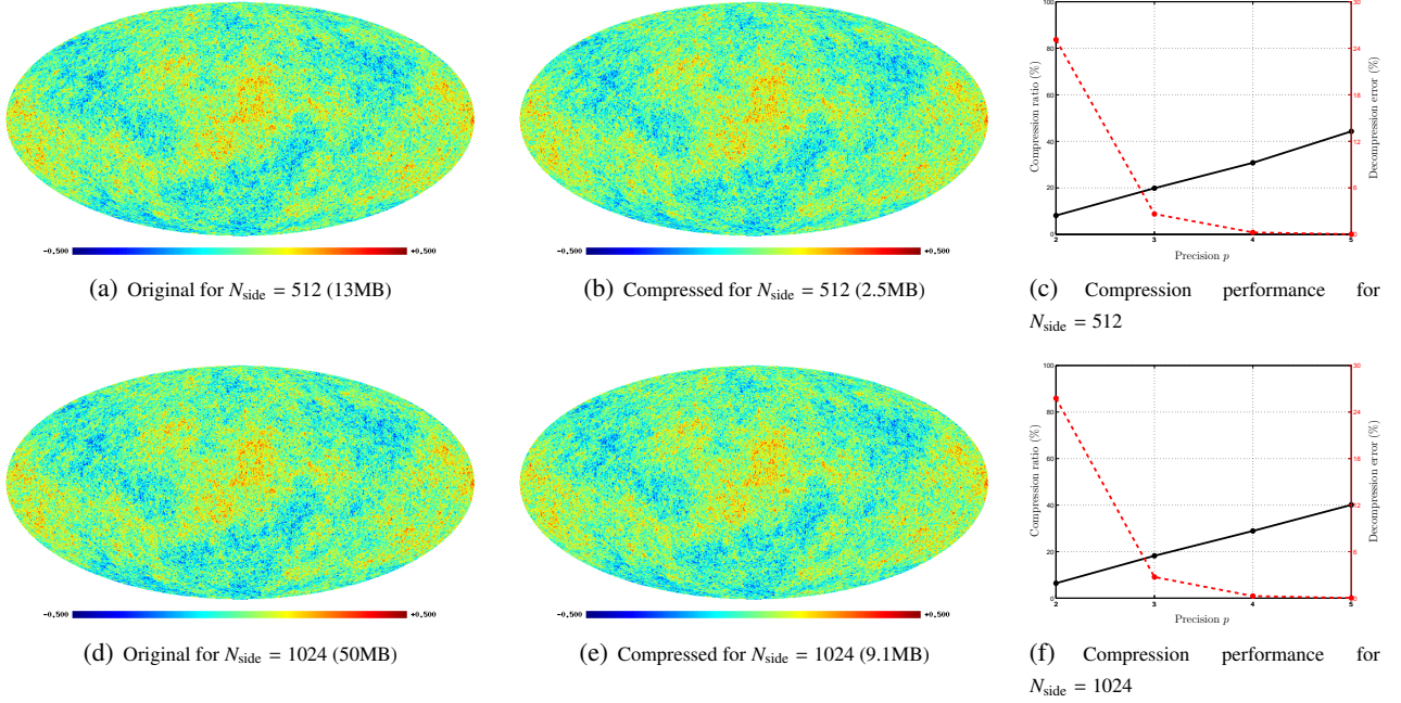
Figure 4. Lossless compression of simulated Gaussian CMB data. The top row of panels shows the compression performance for CMB data with a WMAP resolution of N_{\text{side}} = 512 ( J = 9 ; N \approx 3 \times 10^6 ), while the second row corresponds to CMB data with resolution N_{\text{side}} = 1024 ( J = 10 ; N \approx 13 \times 10^6 ). The first column of panels shows the original simulated CMB data, with corresponding file sizes also specified. The second column of panels shows the CMB data reconstructed from the compressed files for a precision parameter of p = 3 , with corresponding file sizes also specified. It is almost impossible to distinguish by eye any error between the images in the first and second column of panels for this precision parameter (and more difficult as the precision parameter increases). The third column of panels shows the trade-off between compression ratio and decompression fidelity with precision parameter p . Compression ratio (solid black line; left axis) is defined by the ratio of the compressed file size relative to the original file size, expressed as a percentage. The decompression error (dashed red line; right axis) is defined by the ratio of the MSE between the original and decompressed data relative to the RMS value of the original data, expressed as a percentage.
