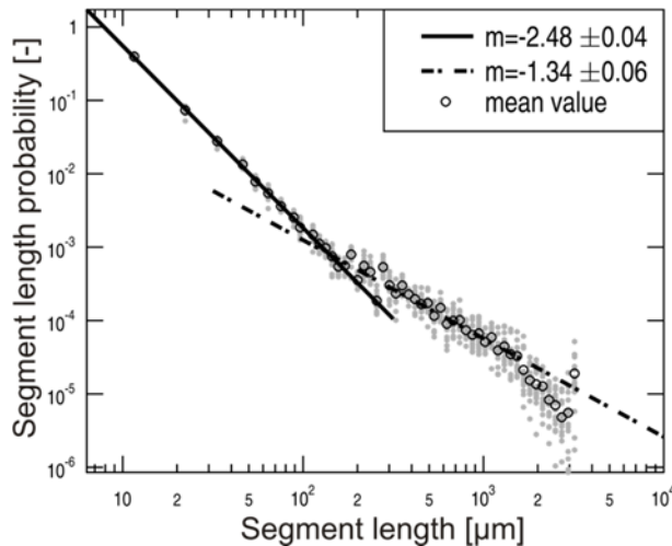
Figure 5: Log-log plot of the normalized distribution of segment length probability.
