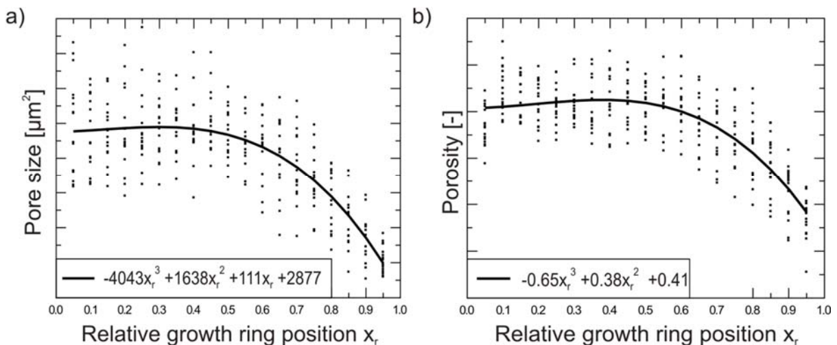
Figure 2: Pore sizes (a) and porosities (b) as a function of a dimensionless relative position in the growth ring (in which: 0.0 represents earlywood and 1.0 represents latewood). The polynomial equations describe the correlation curves presented.
