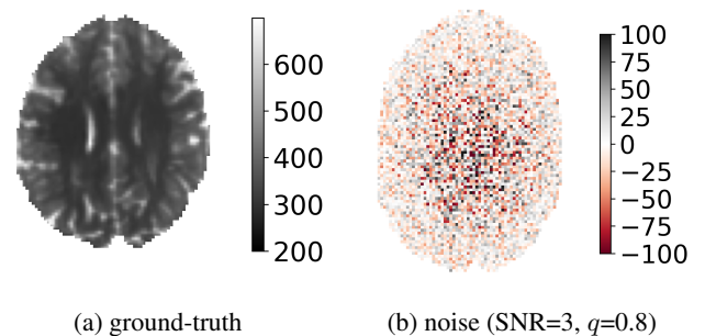
Fig. 2: Synthetic dataset.
