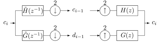
Fig. 1. Analysis-synthesis filterbank for the 1-D nonredundant wavelet decomposition.
